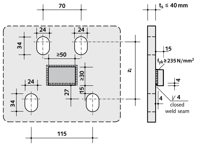
Hole layout for HIT-SMV with M22 thread (HIT-HP/SP SDV-2M22, HIT-HP/SP SMV-2M22)
